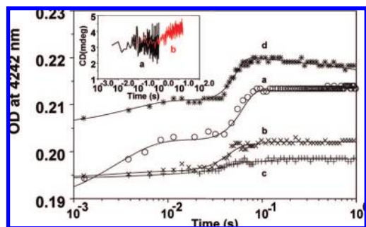
Figure 4. Kinetic progress curves for the interaction of CuT4 with (curve a) PheA by simple mixing, (curve b) PheA after 15 ms of exposure to TPPS, (curve c) PheA after 150 ms of exposure to TPPS, and (curve d) PheA after full equilibration (i.e., 20 min) with TPPS. Individual curves have been displaced for a better comparison.
